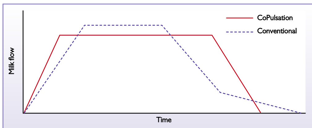
Fig. 1. Comparison of the milk flow rates achieved with a conventional pulsation system and the CoPulsation milking system. CoPulsation is a trademark of LR Gehm LLC.
