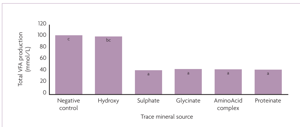
Fig. 1. Total Volatile Fatty Acid (Total VFA) production during an in vitro fermentation trial where a negative control fermentation substrate was supplemented with five different sources of trace elements (P<0.05 for different superscripts).
